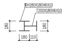
GKZ2(实H180X180X6X10+T200X180X6X10)
