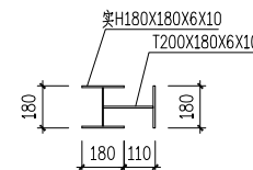
GKZ1 (实H180X180X6X10+T200X180X6X10)
