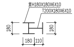
GKZ1(实H180X180X6X10+T200X180X6X10)
